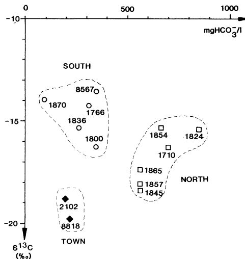
Fig 3. δ 13 C values for the DIC of groundwater samples from the Jakarta district vs bicarbonate concentration
