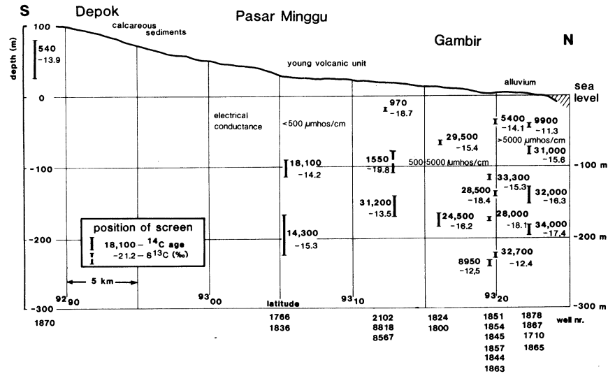
Fig 2. Conventional 14 C ages and δ 13 C values of representative groundwater samples from the Jakarta City District vs sampling depth (after Wandowo, Manurung & Zainal, 1985)
